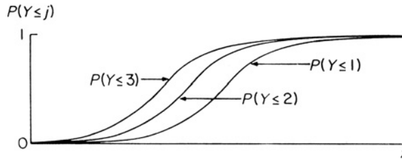
Figure 6.2 Depiction of cumulative probabilities in the cumulative logit model.
