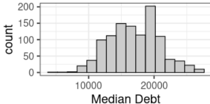
Bimodal
